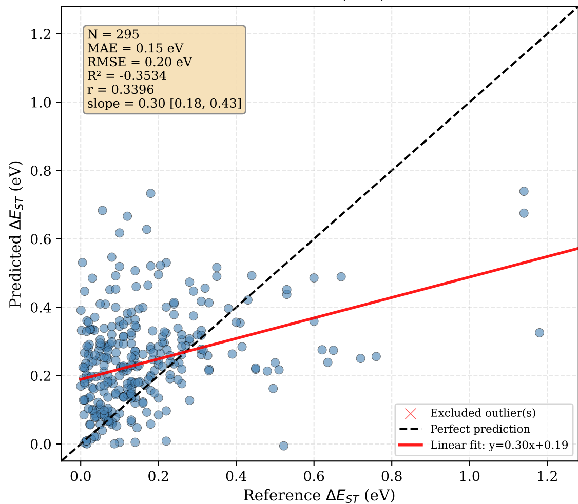
sTD-DFT (Tol)
