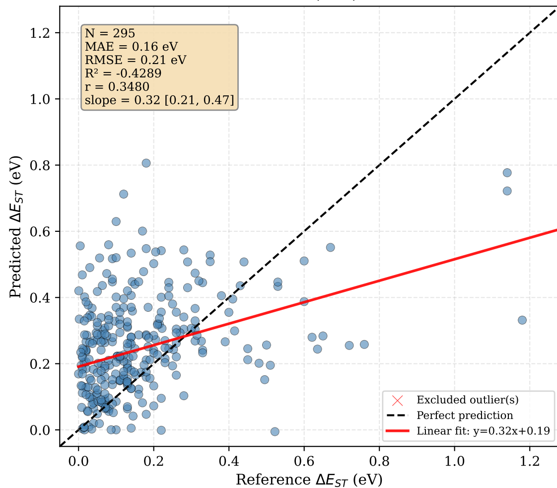
sTDA (Tol)
