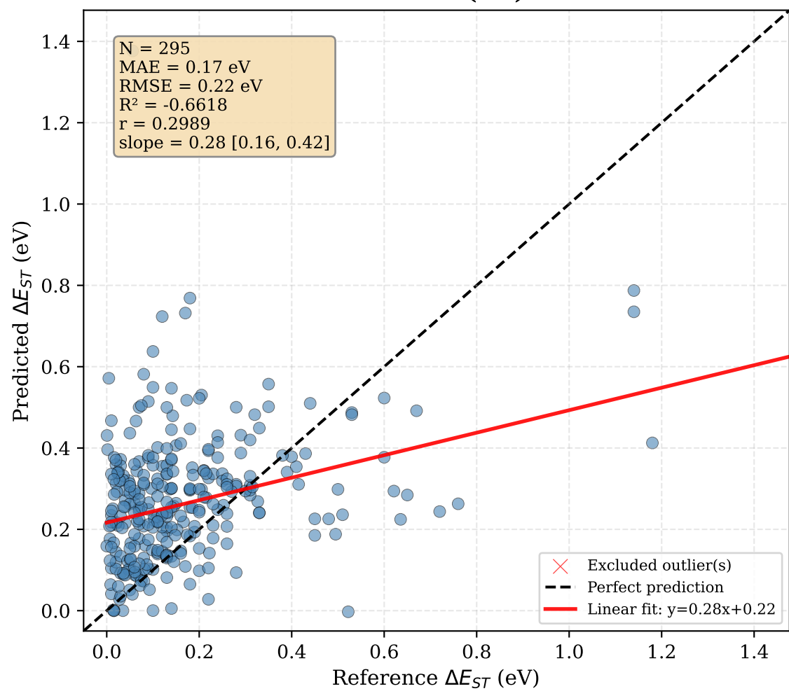
sTD-DFT (Tol)
